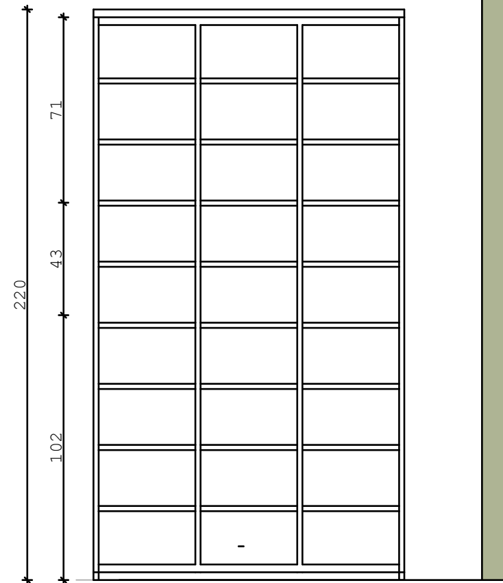
ALZADO INTERIOR ARMARIO ZAPATERO
